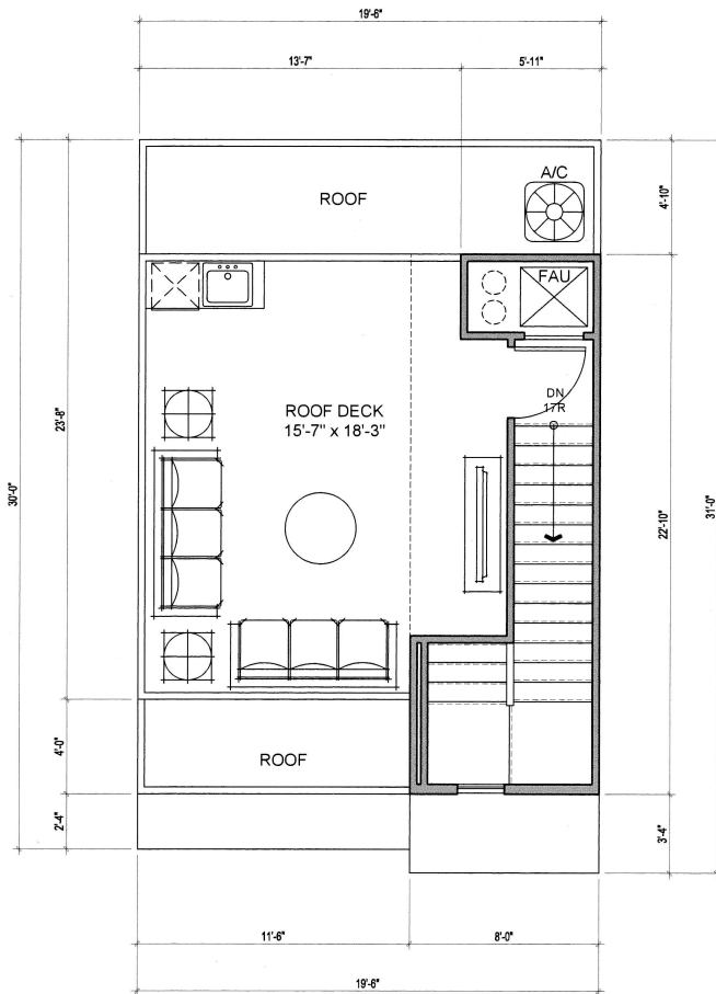
ROOF DECK
